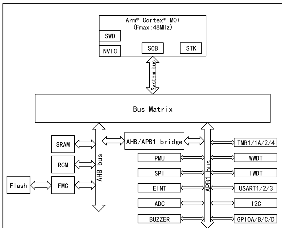
Figure 1 System Architecture of APM32A003F6Ux Series Products
