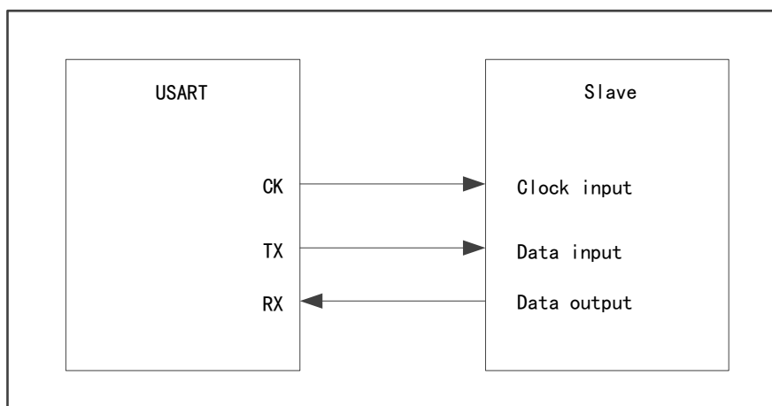
Figure 52 USART Synchronous Transmission Example
