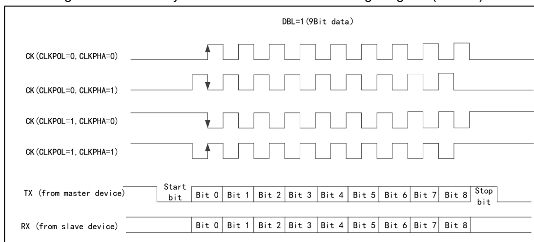
Figure 54 USART Synchronous Transmission Timing Diagram (DBL=1)
