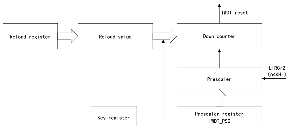
Figure 42 Independent Watchdog Block Diagram
