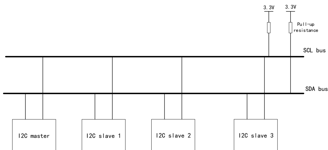
Figure 61 Commonly Used I2C Communication Connection Diagram
