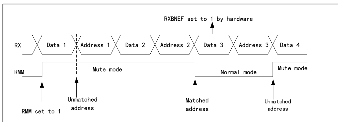
Figure 51 Address Flag Exit Mute Mode
