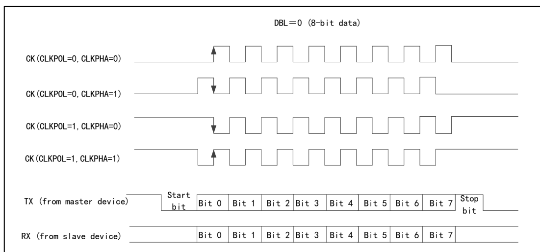
Figure 53 USART Synchronous Transmission Timing Diagram (DBL=0)
