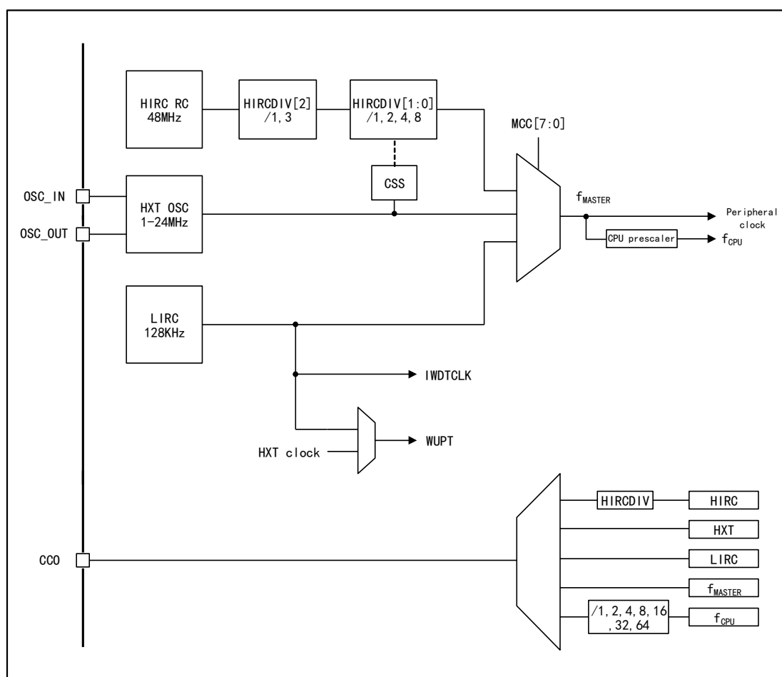
Figure 7 APM32A003F6Ux Clock Tree
